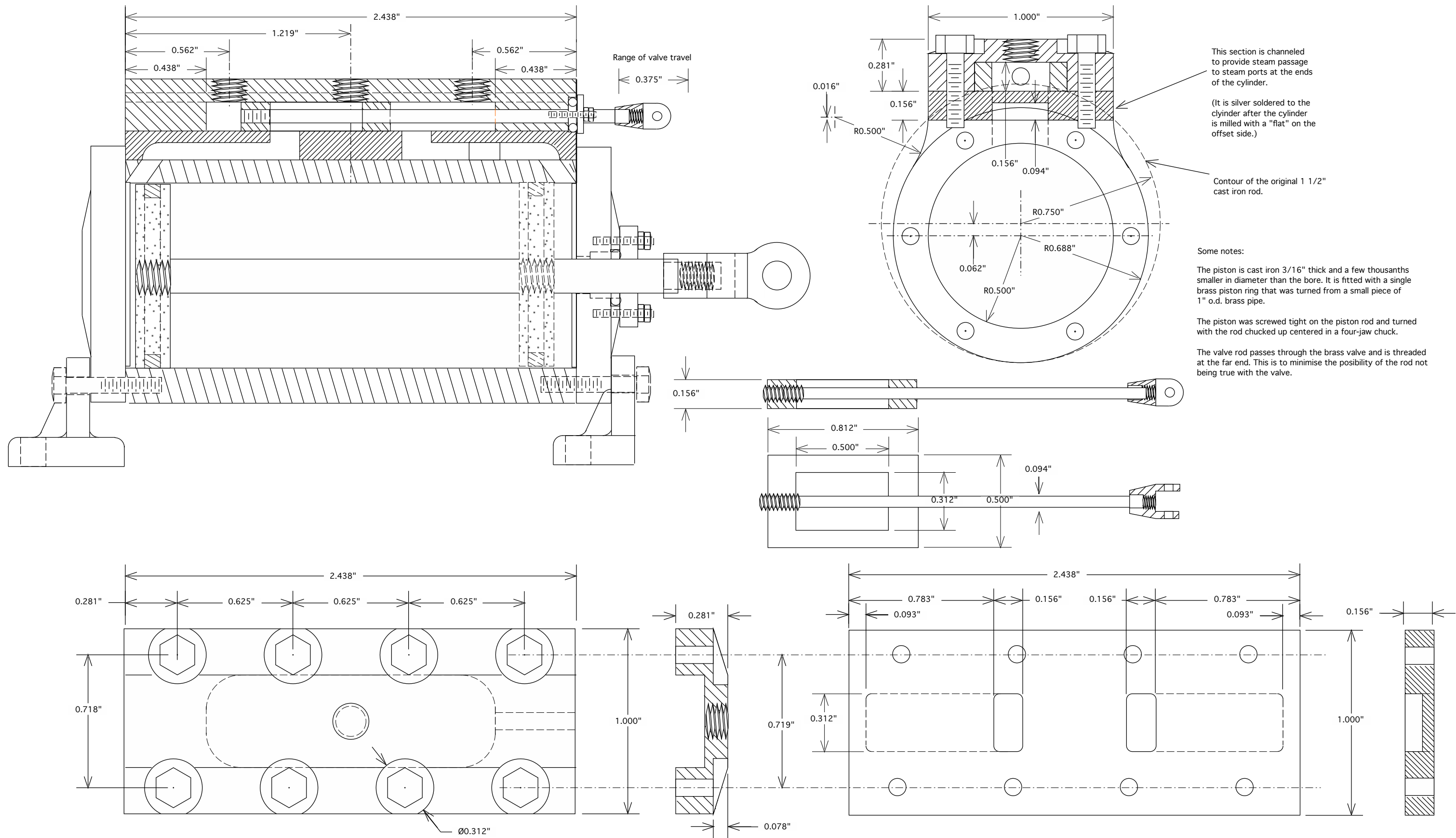
The top view shows the slide valve above the cylinder bore, with an end view to its right. The slide valve itself is shown in side and top views. The steam chest cover is shown at the bottom in top and end views. To the right is shown the steam ports and channels in a plate soldered to a flat milled on the top of the cylinder body.
