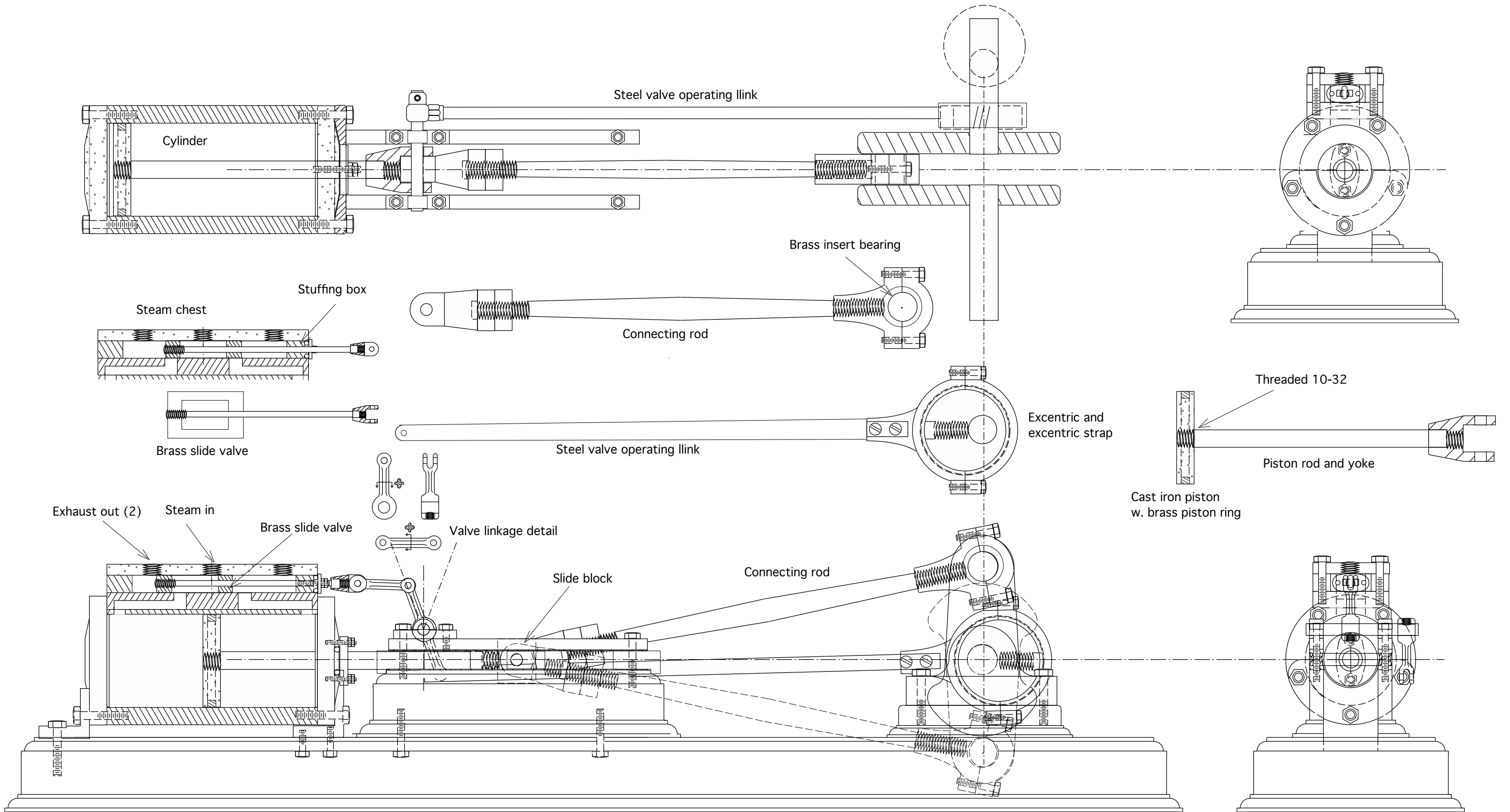
Top view is of the engine showing the crosshead, connecting rod, valve rock shaft, and crankshaft. The bottom view is of the engine from the side showing the valve linkage and the crank in mid rotation. In the crank position shown at the top, the slide valve is all the way to the left selecting the left port for steam entry to the left side of the piston. The right side of the piston is open to exhaust.
